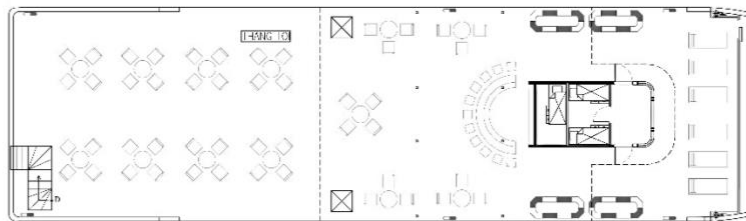
Sundeck Floor - Khu bong tau
